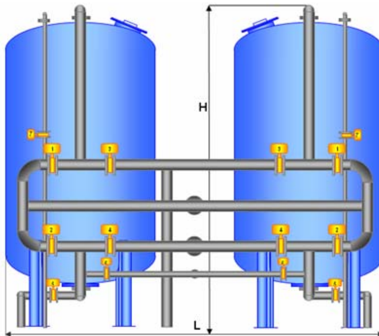
DIMENSION OF STANDARD TANDEM SAND FILTRATION UNIT (ESF1-SERIES)
